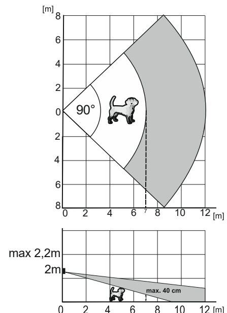
Figure 3.: Detection characteristics
